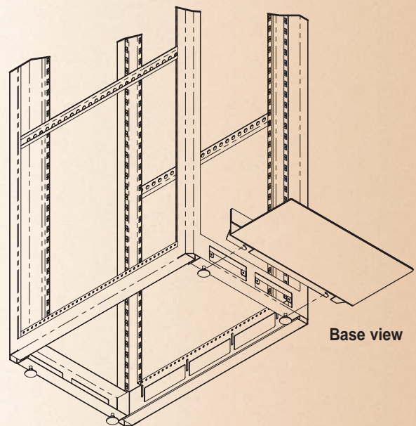
Full cabinet view excluding panels
